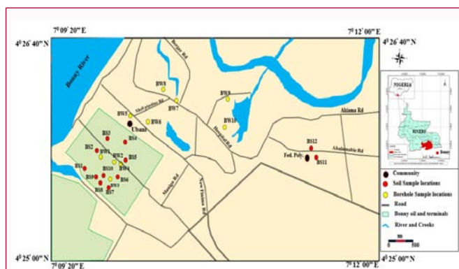
Figure 1: Map of the study area showing soil and groundwater sampling locations in Bonny.
