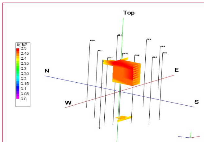
Figure 7: 3-D block model showing the horizontal and vertical variations in BTEX concentration around the spill area after applying the DPR target value (0.4 mg/kg) as a cutoff (Volume 40,000m³).
