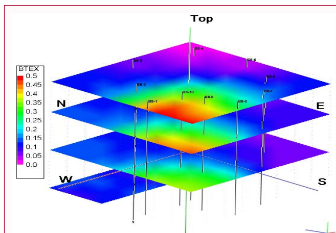
Figure 6: Depth slices extracted from the 3-D BTEX grid model at 0.1m, 0.5m, 1.0m and 1.5m around the spill area.
