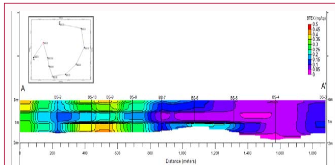
Figure 5: A cross-section across the entire wells showing BTEX variations with depth.
