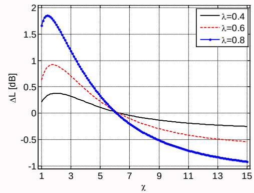
Figure 4: Dependence of the error \Delta L (Eqs. 20,21) on the relative distance, \chi = d/h , relative blade length, \lambda = l/h (Figure 1), and the ground parameter, \gamma = 0.01 (Table 1).
