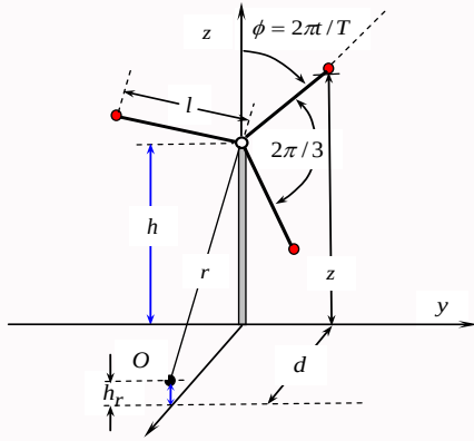
Figure 1: Blade tips as a sound sources rotating with the angular frequency \omega = 2\pi/T . The receiver O is close to the x-axis ( h_r \ll d ).
