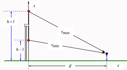
Figure 3: The longest and shortest distances from a rotating tip to the receiver, r_{\max} and r_{\min} (Eq.7).
